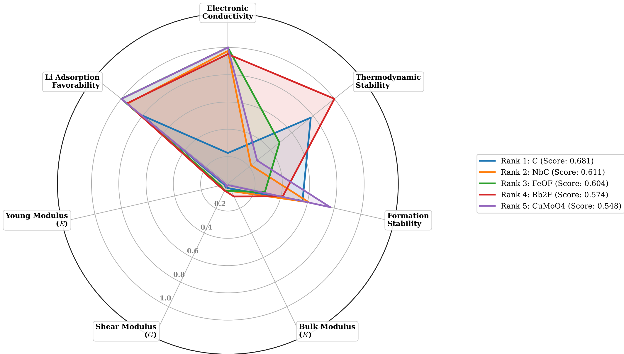
Holistic 7-Axis Performance Radar Map for Top 5 Candidate Anode Materials
